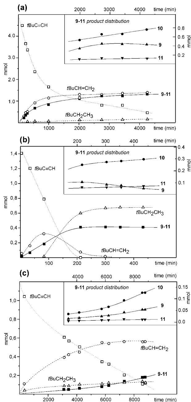
Figure 2. Reaction profiles for t -BuC≡CH hydrogenations catalyzed by 1 . Conditions: (a) 1,2-dichloroethane (8 mL), 293 K, [1] 0 = 0.010 mmol, [ t -BuC≡CH] 0 = 5.0 mmol, P (H 2 ) = 1.1 bar; (b) 1,2-dichloroethane (8 mL), 293 K, [1] 0 = 0.015 mmol, [ t -BuC≡CH] 0 = 1.5 mmol, P (H 2 ) = 1.1 bar; (c) toluene (6 mL), BMIM·BF 4 (2 mL), 293 K, 1 = 0.019 mmol, [ t -BuC≡CH] 0 = 1.19 mmol, P (H 2 ) = 1.1 bar.
