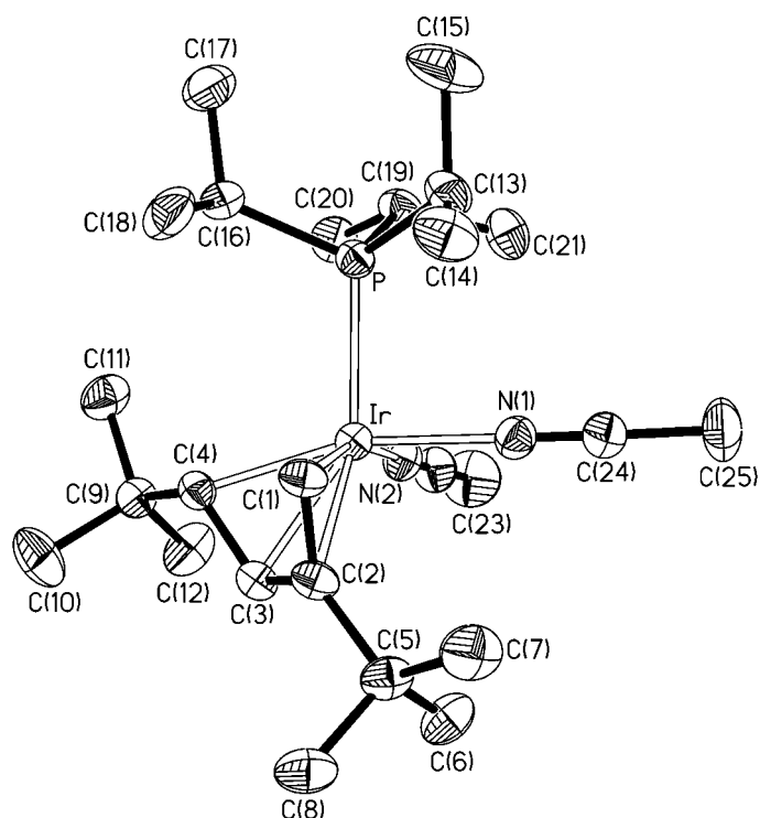
Figure 1. Molecular structure of the cation of complex 5 (ORTEP). Selected bond distances [Å] and angles [°]: Ir–P 2.3559(12), Ir–N1 2.1000(4), Ir–N2 2.090(4), Ir–C1 2.111(4), Ir–C2 2.193(4), Ir–C3 2.179(4), Ir–C4 2.151(4); C1–C2–C3 113.3(4), C2–C3–C4 118.6(4), C3–C4–C9 118.1(4).
