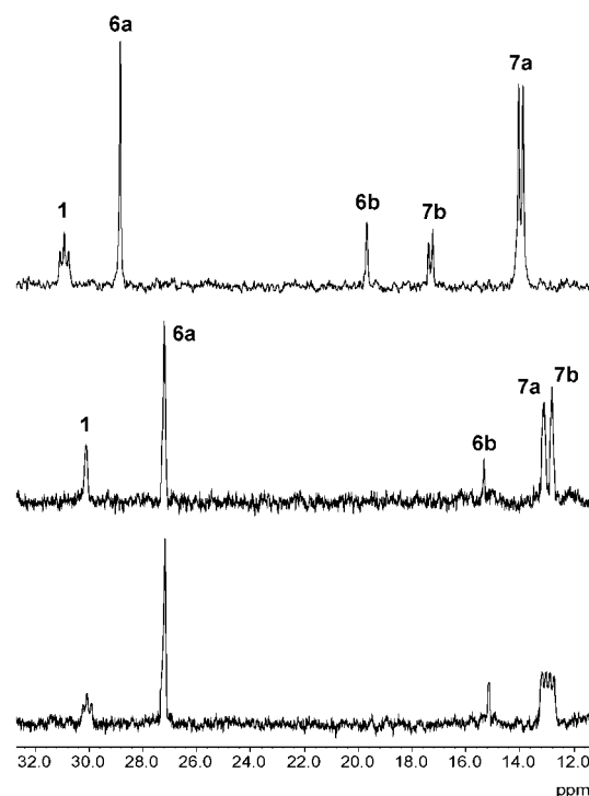
Figure 3. 31 P NMR spectra of compound mixtures obtained by treatment of 1 with PhC≡CH at room temperature: (above) 31 P off resonance spectrum in CDCl 3 ; (center) 31 P{ 1 H} spectrum in BMIM·BF 4 ; (below) 31 P off resonance spectrum in BMIM·BF 4 .
